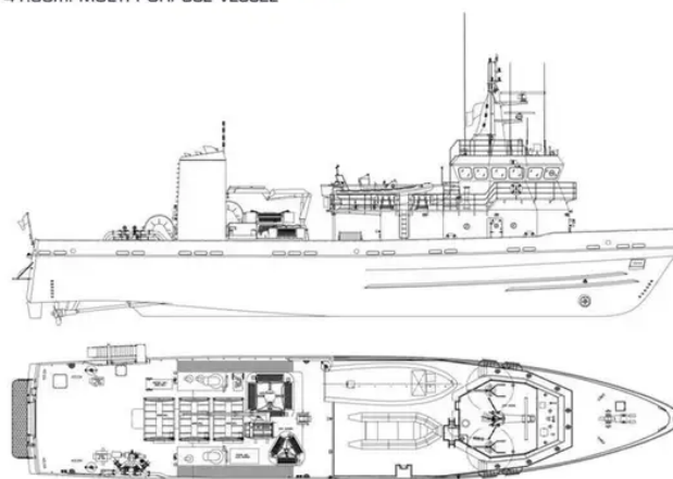
41.85m. MULTI PURPOSE VESSEL
